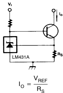
Figure 16. Constant-Current Sink
