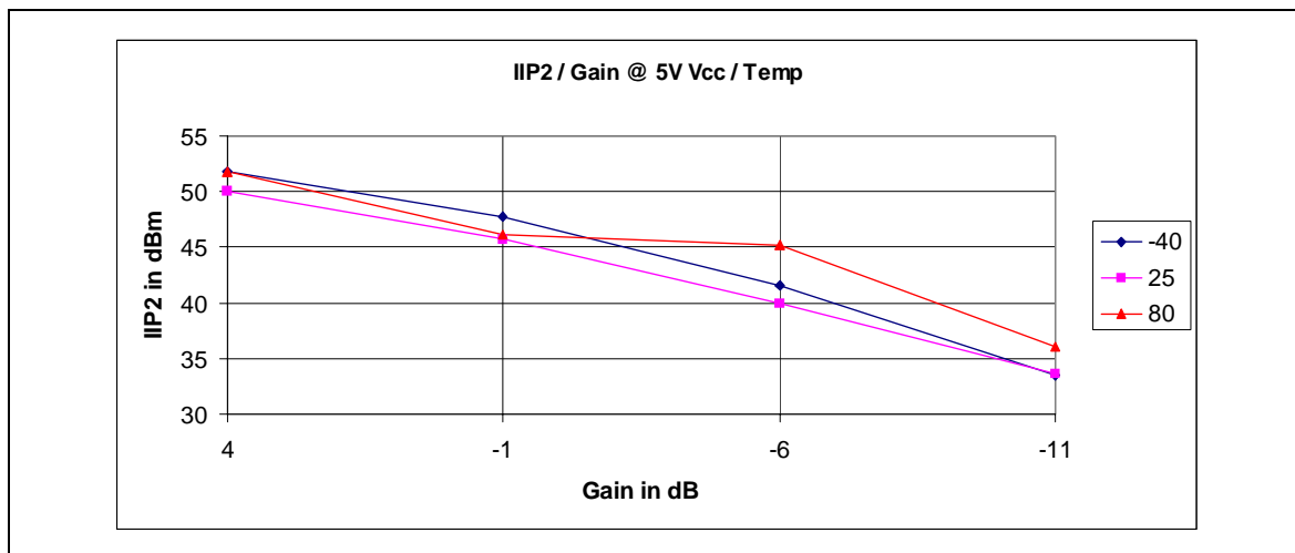
Figure 23 - Typical IIP2 / Gain @ 5V Vcc / Temp @ 500MHz
