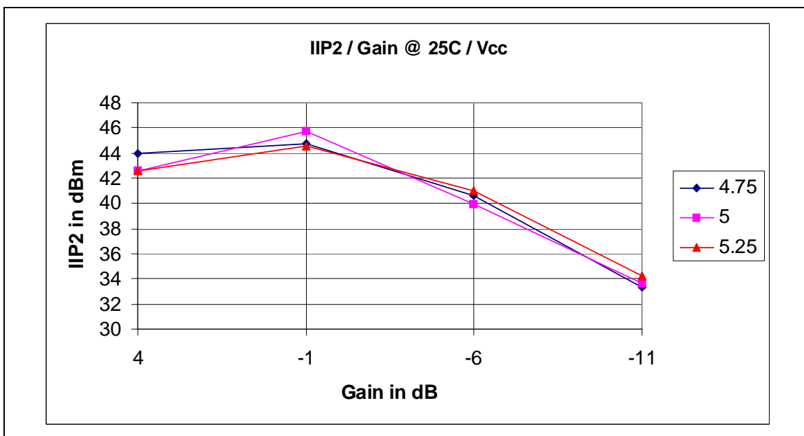
Figure 22 - Typical IIP2 / Gain @ 25C / Vcc @ 500MHz
