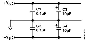
Figure 58. Supply Bypassing
