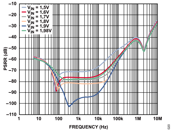
Figure 20. Power Supply Rejection Ratio (PSRR) vs. Frequency for Various V_{IN} , V_{OUT} = 1.3\text{ V} , Load Current = 1 A
