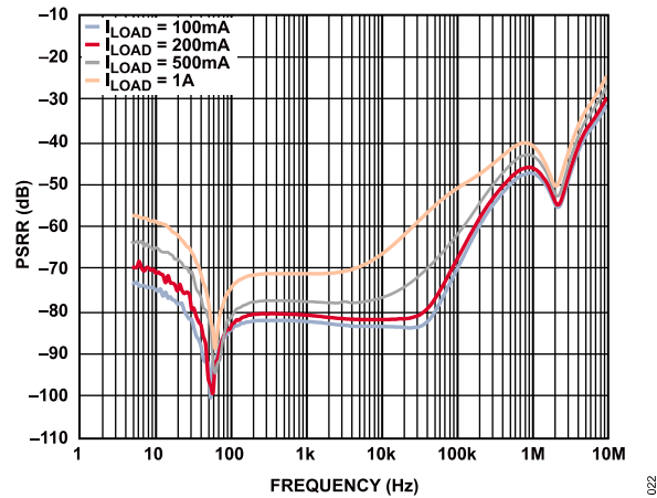
Figure 22. Power Supply Rejection Ratio (PSRR) vs. Frequency for Various Loads, V_{OUT} = 1.3\text{ V} , V_{IN} = 1.5\text{ V}
