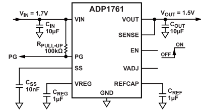
Figure 1. Fixed Output Operation
