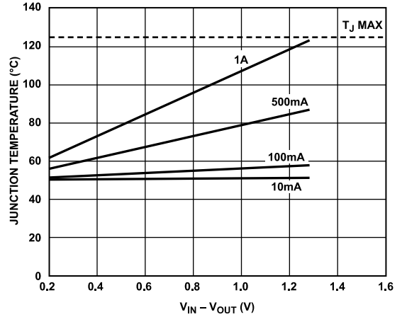
Figure 37. 6400 mm 2 of PCB Copper, T A = 50°C
