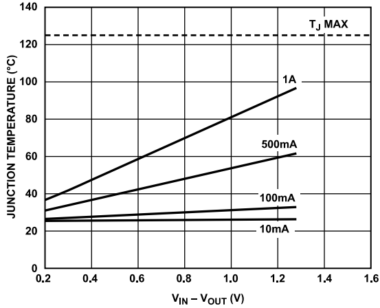
Figure 34. 6400 mm 2 of PCB Copper, T A = 25°C
