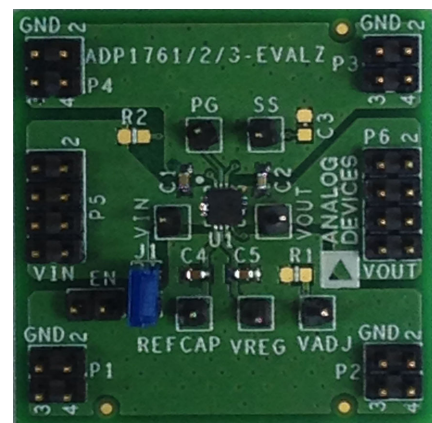
Figure 44. Evaluation Board
