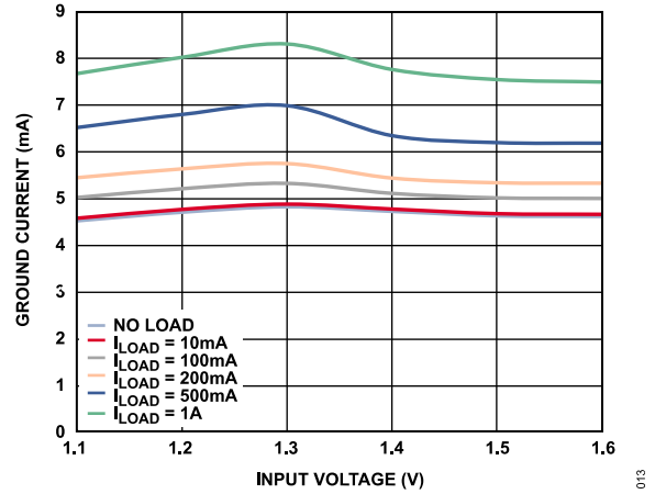
Figure 13. Ground Current ( I_{GND} ) vs. Input Voltage ( V_{IN} ) (in Dropout), V_{OUT} = 1.3 V
