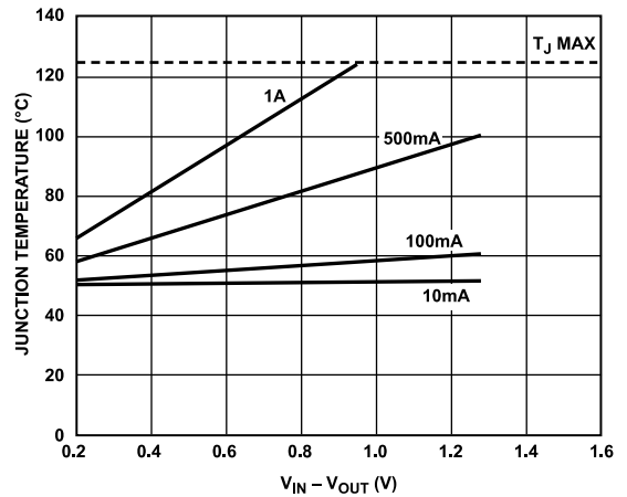
Figure 38. 500 mm 2 of PCB Copper, T A = 50°C
