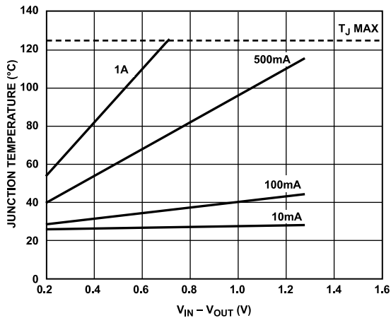
Figure 36. 25 mm 2 of PCB Copper, T A = 25°C
