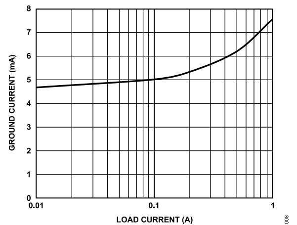
Figure 8. Ground Current ( I_{GND} ) vs. Load Current ( I_{LOAD} )
