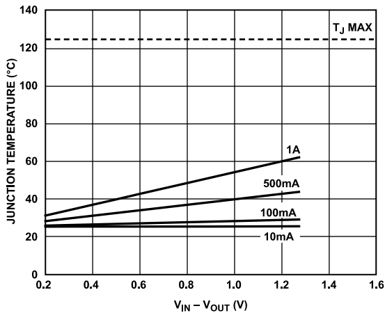
Figure 42. 1000 mm 2 of PCB Copper, T_B = 25^\circ\text{C}
