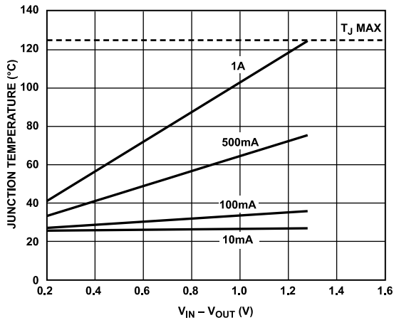
Figure 35. 500 mm 2 of PCB Copper, T A = 25°C
