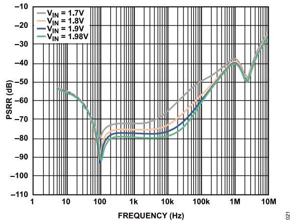
Figure 21. Power Supply Rejection Ratio (PSRR) vs. Frequency for Various V_{IN} , V_{OUT} = 1.5\text{ V} , Load Current = 1 A
