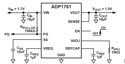
Figure 2. Adjustable Output Operation
