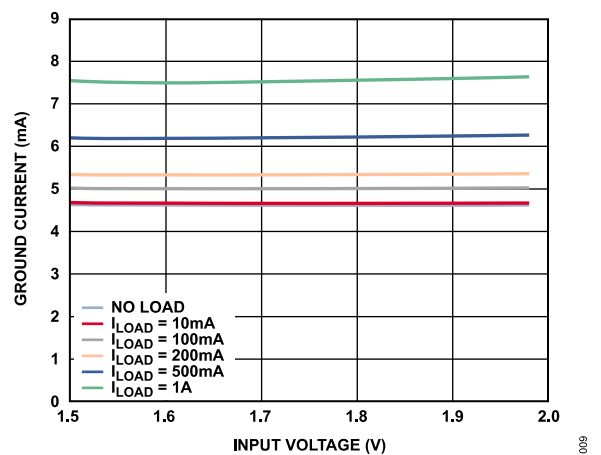
Figure 9. Ground Current ( I_{GND} ) vs. Input Voltage ( V_{IN} )
