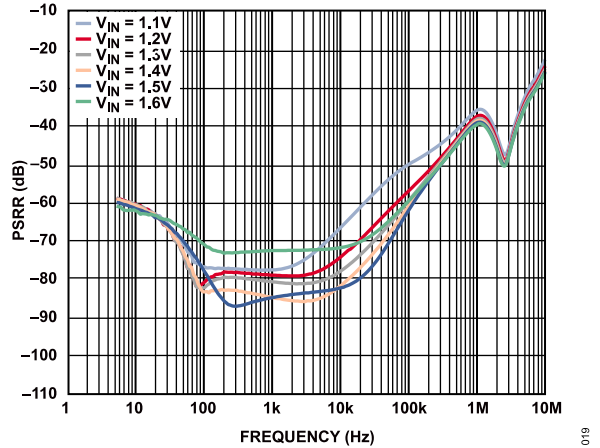
Figure 19. Power Supply Rejection Ratio (PSRR) vs. Frequency for Various V_{IN} , V_{OUT} = 0.9\text{ V} , Load Current = 1 A
