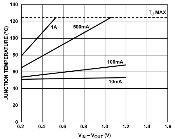
Figure 39. 25 mm 2 of PCB Copper, T A = 50°C
