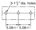
<PCB Mounting Dimensions (Reference)>
