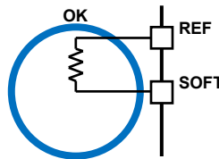
Resistor Pull-up
