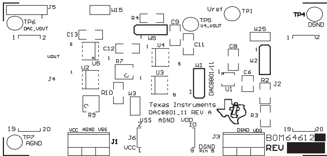
Figure 2. Top Silkscreen
