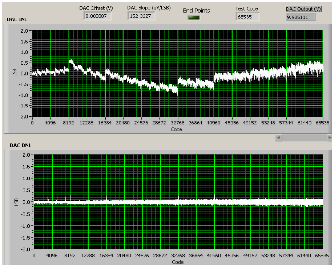
Figure 8. INL and DNL Characterization Plot for the DAC8811
