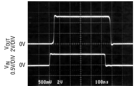
Output-Overload Recovery
