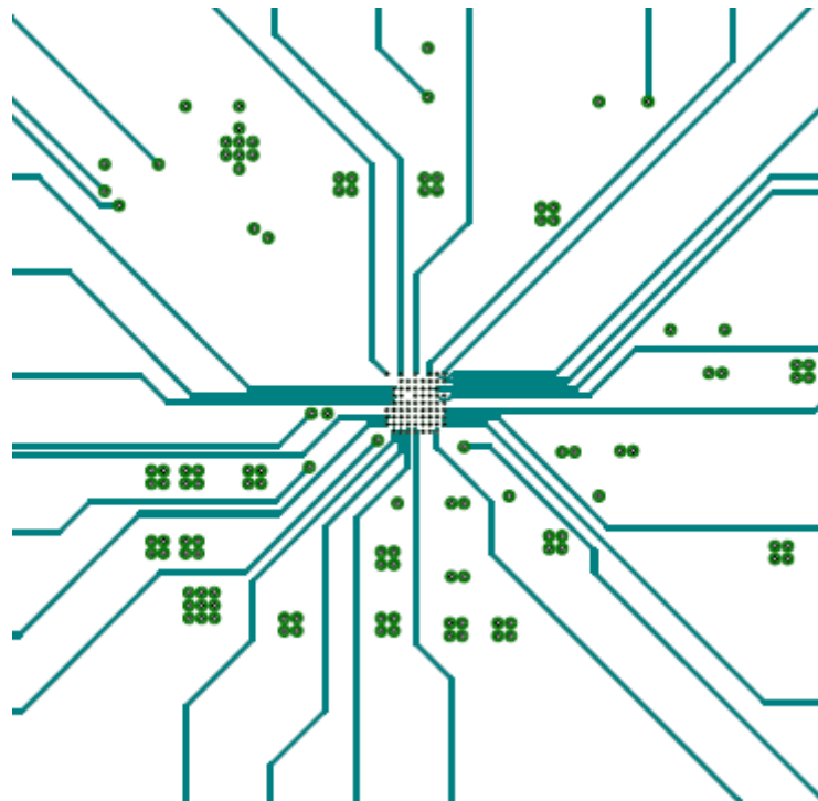
Figure 45. PCB Layout Image (Mid1 Layer)
