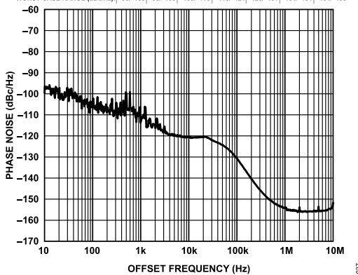
Figure 37. Phase Noise Performance Including Distribution Table at LO Frequency = 100 MHz at Nominal and Worst-Case Conditions
