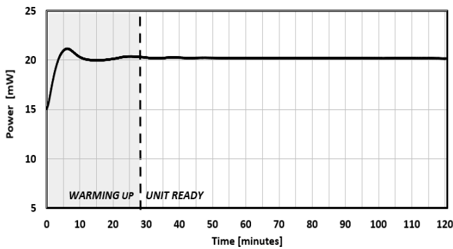
FIG. 9: WARM-UP TIME
