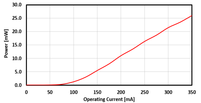
FIG. 10: SLED 3 OUTPUT POWER VS CURRENT
