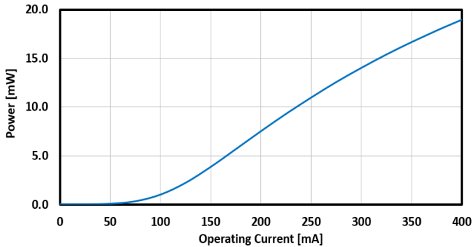
FIG. 11: SLED 4 OUTPUT POWER VS CURRENT
