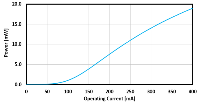
FIG. 12: SLED 5 OUTPUT POWER VS CURRENT
