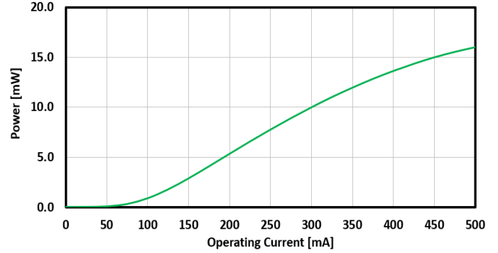
FIG. 8: SLED 1 OUTPUT POWER VS CURRENT
