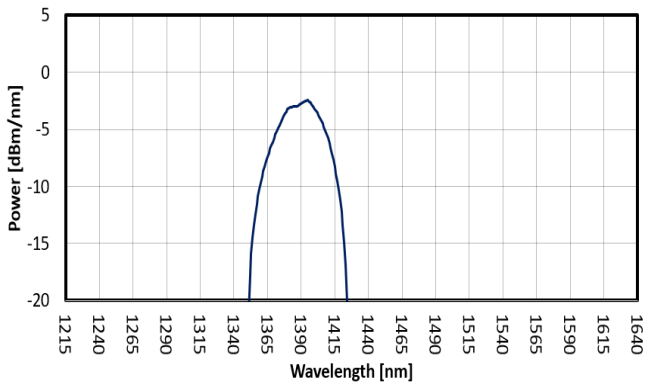
FIG. 5: SLED 4 SPECTRUM
