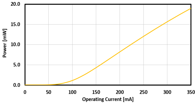
FIG. 9: SLED 2 OUTPUT POWER VS CURRENT
