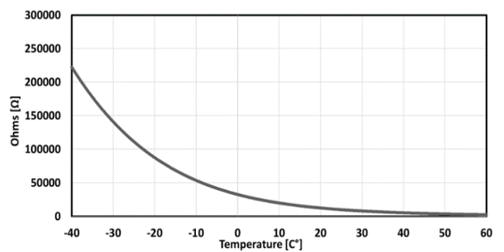
FIG. 14: THERMISTOR R_{\text{THTEC}} RESISTANCE VS TEMPERATURE
