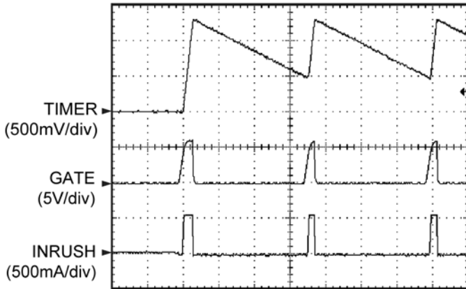
Time (25ms/div)
