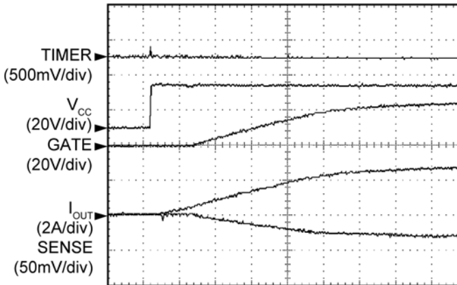
Time (10ms/div)
