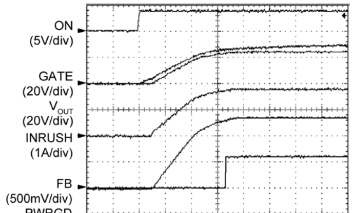
Time (10ms/div)
