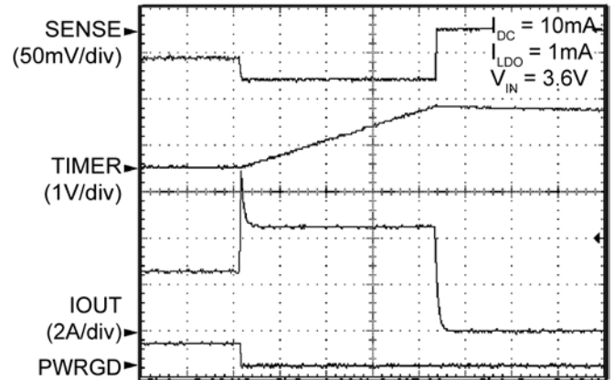
Time (5ms/div)
