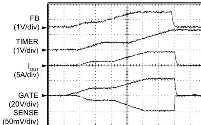
Time (5ms/div)
