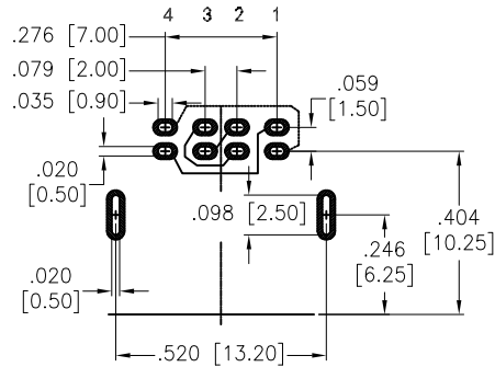
RECOMMENDED PCB LAYOUT (MULTIPLE LAYER)
