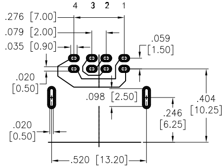
RECOMMENDED PCB LAYOUT (SINGLE LAYER)
