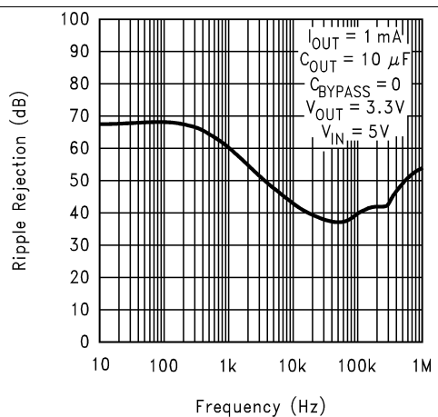
Figure 6. Ripple Rejection
