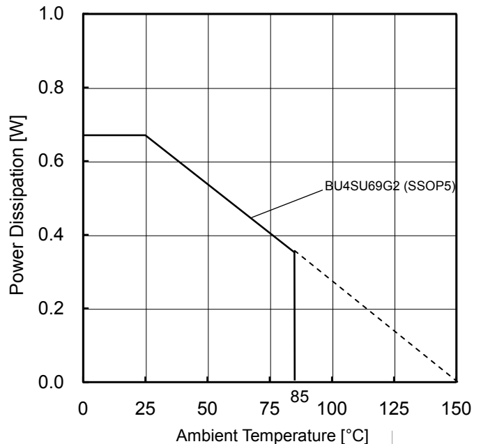
Figure 12. Derating Curve
