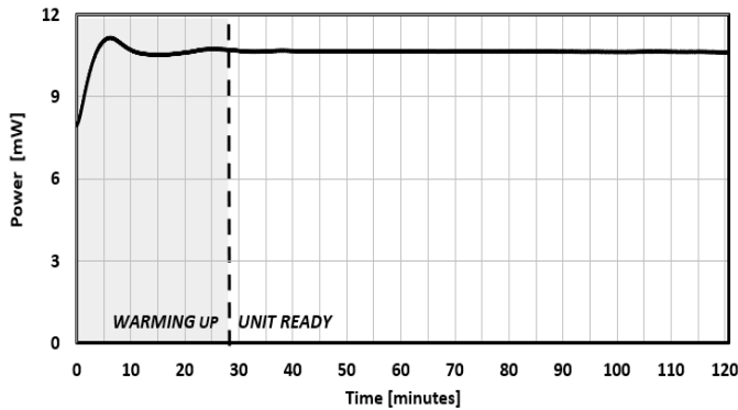
FIG. 7: WARM-UP TIME
