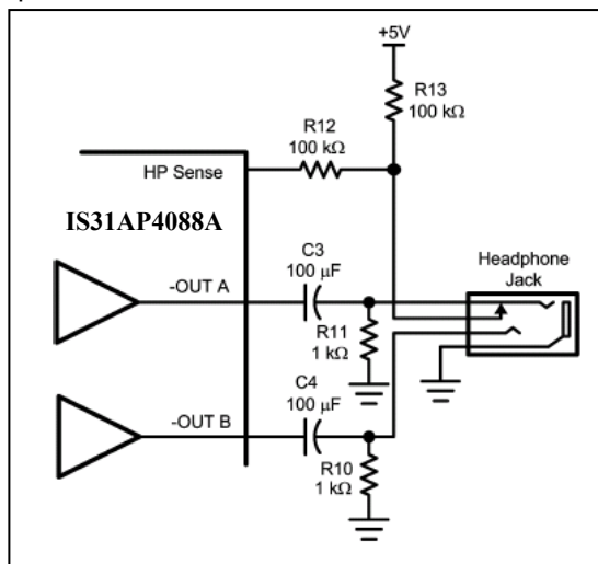
Figure 33 Headphone Circuit
