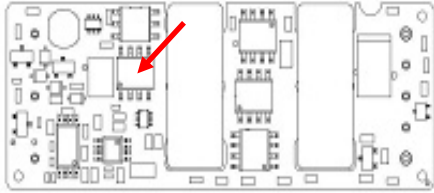
Figure 18. Temperature Monitoring Locations
