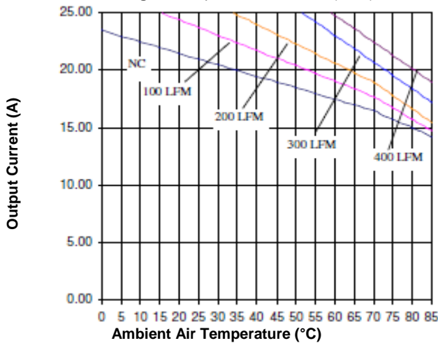
Figure 11. Current Derating Curve for Airflow Direction 3 (Ref. Fig. 12 for Airflow Direction; V_{in} = 48V, open frame)
