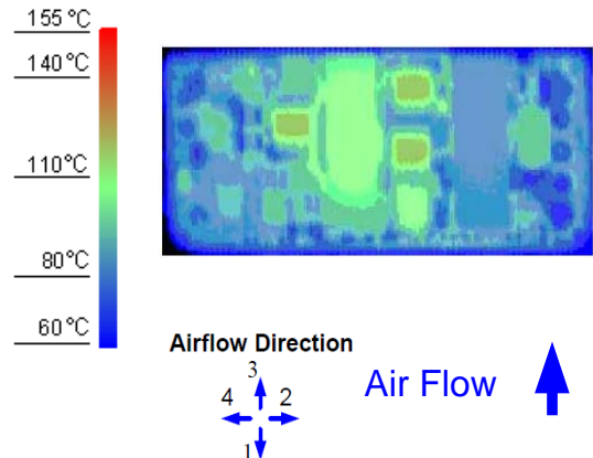
Figure 12. Thermal Image for Airflow Direction 3 (21A output, 55°C ambient, 200 LFM, typical V_{in} , open frame, socket interface)
