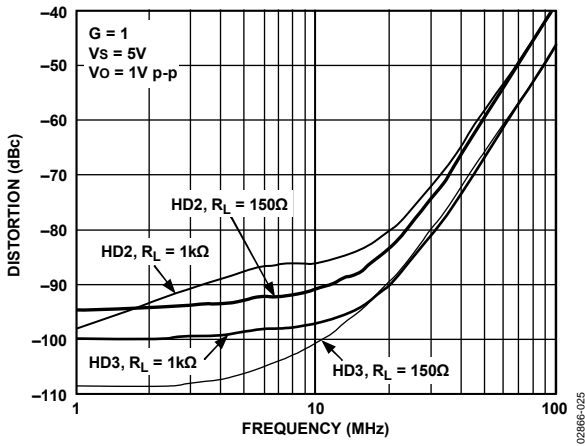
Figure 25. AD8008 Second and Third Harmonic Distortion vs. Frequency and R_L
