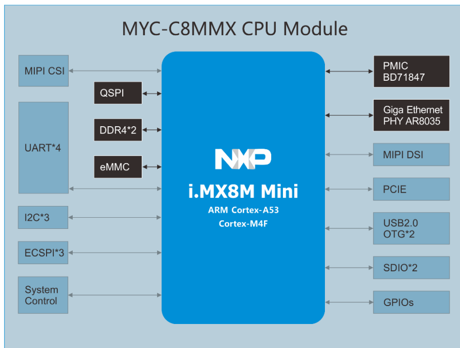
Figure 1-9 MYC-C8MMX CPU Module Function Block Diagram
