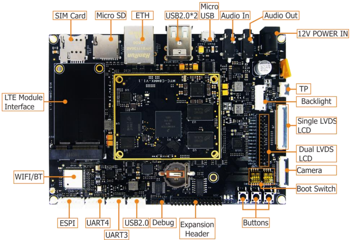
Figure 1-3 MYD-C8MMX Development Board Top-view
