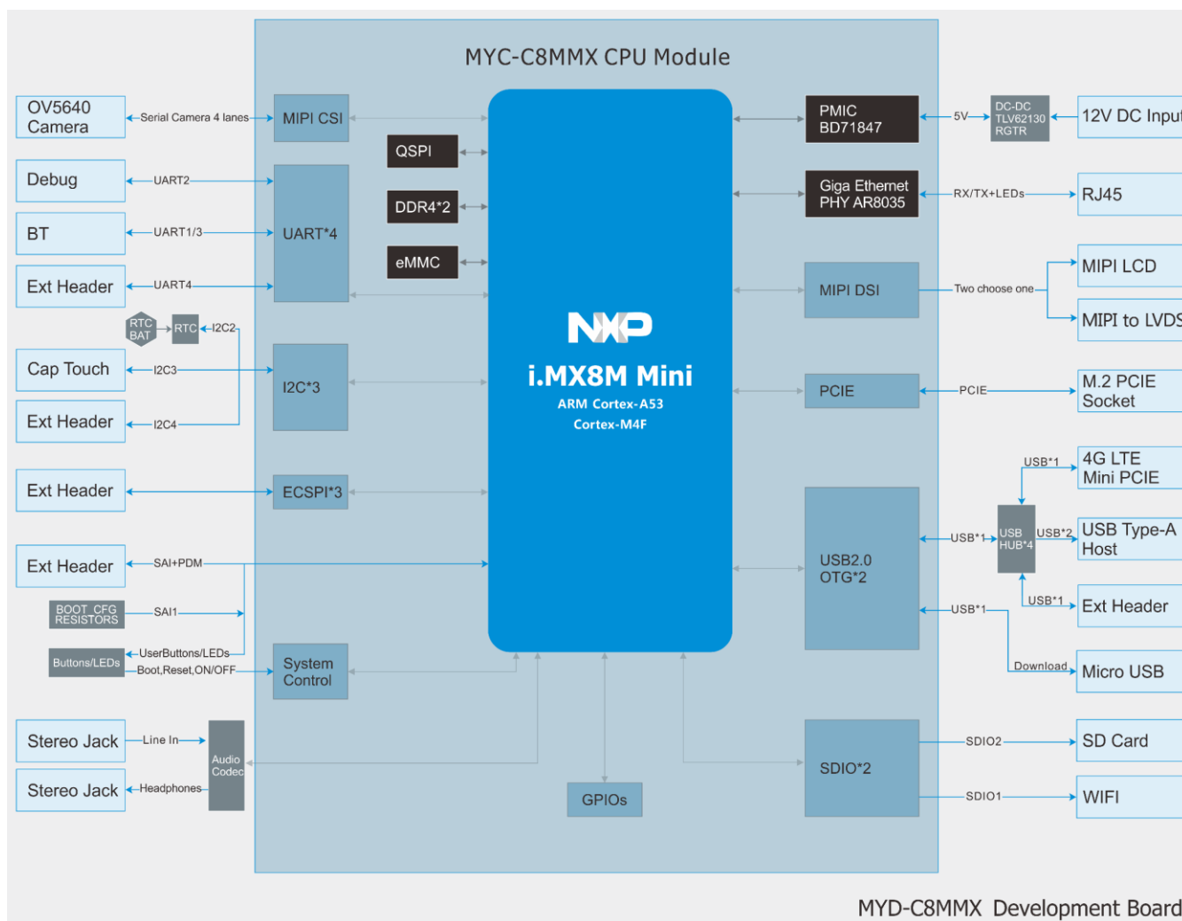
Figure 1-10 MYD-C8MMX Development Board Function Block Diagram
