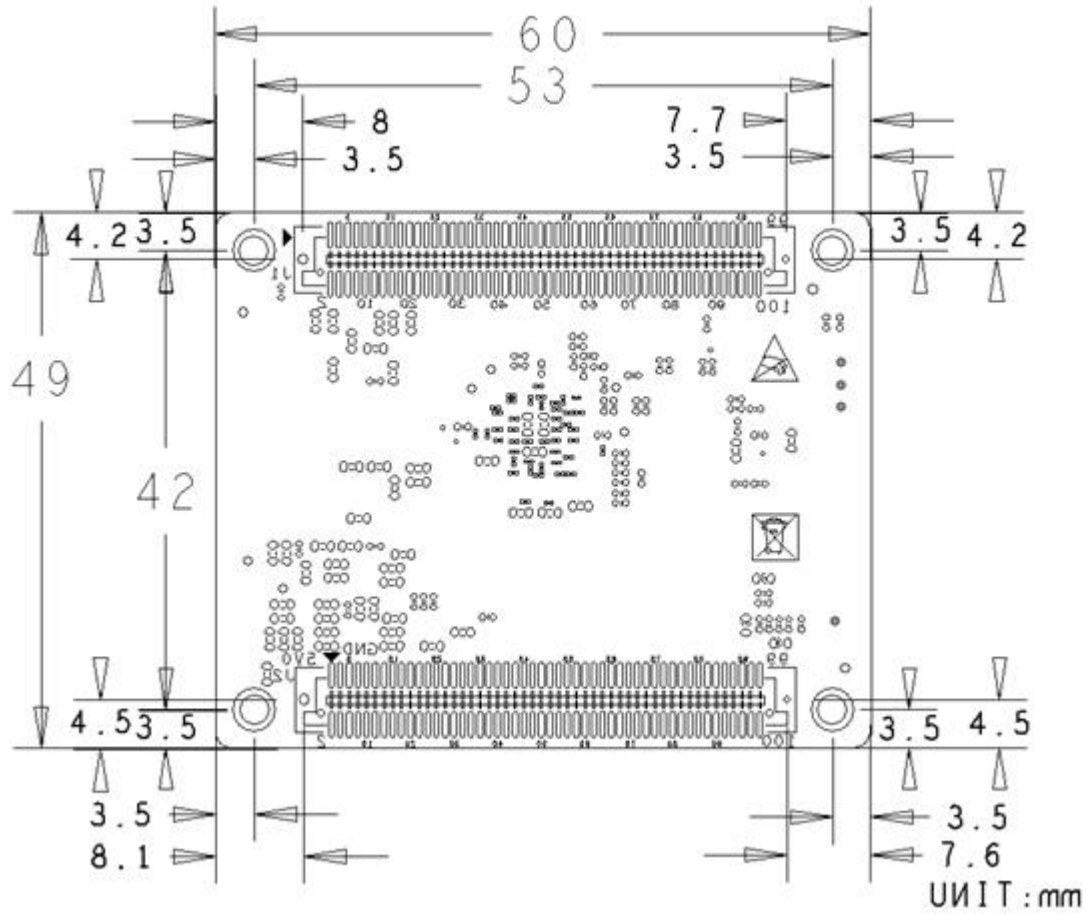
Figure 1-11 MYC-C8MMX Dimensions Chart
