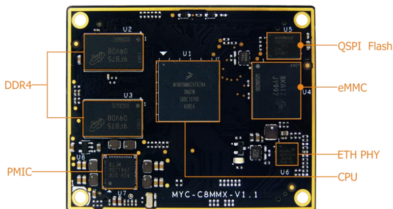
Figure 1-6 MYC-C8MMX CPU Module Top-view
