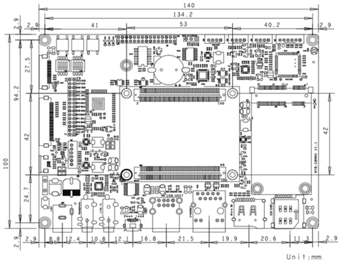
Figure 1-12 MYD-C8MMX Dimensions Chart
