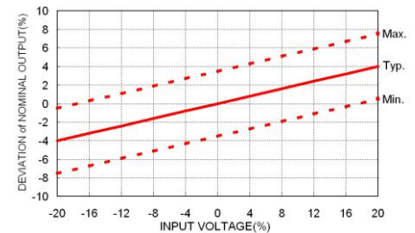
Vout Deviation vs. Input Voltage for 12, 15, 24Vin Models
