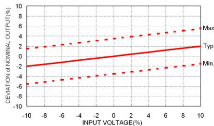
Vout Deviation vs. Input Voltage for 5Vin Models
