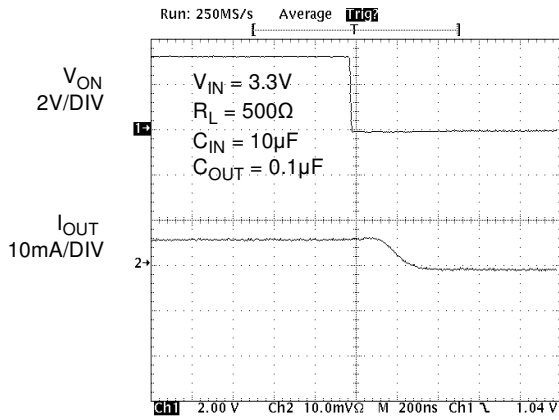
Figure 21. T_{OFF} Response
