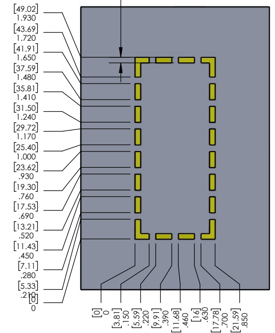
TRACE PATTERN SCALE 1:1
