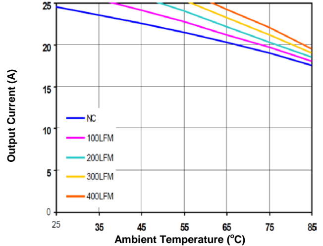
Figure 6b. Current Derating Curve ( V_{in}=12V , open frame)
