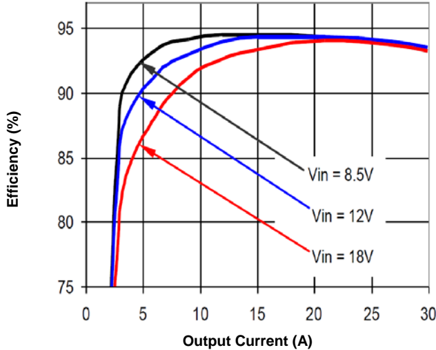
Figure 4a. Efficiency vs. Load Current (25°C)
