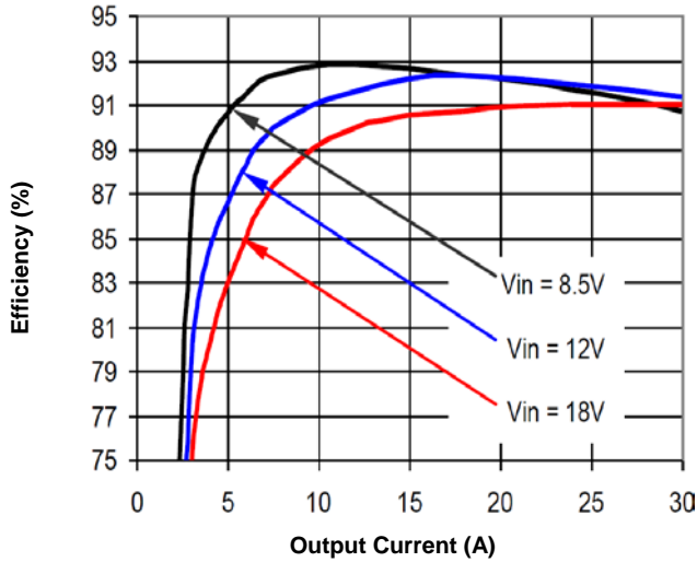
Figure 3a. Efficiency vs. Load Current (25°C)
