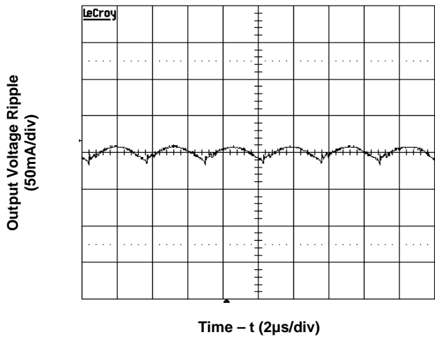
Figure 1c. Output Voltage Ripple (Vin=12V, full load)
