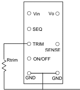
Figure 9. Circuit for Output Voltage Trim
