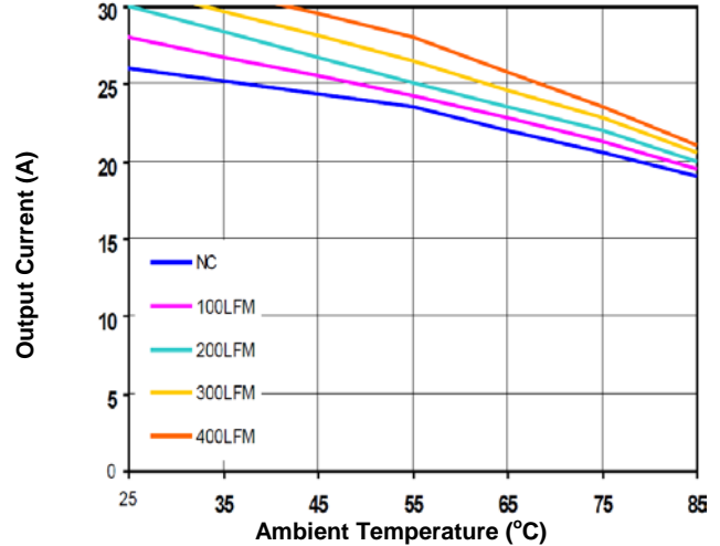
Figure 4b. Current Derating Curve ( V_{in}=12V , open frame)
