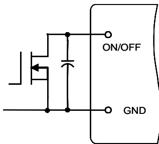
Figure 7. Circuit for Positive Logic Control
