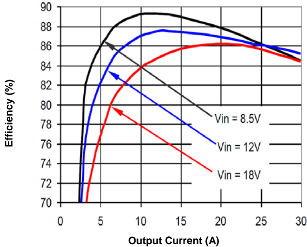
Figure 2a. Efficiency vs. Load Current (25°C)
