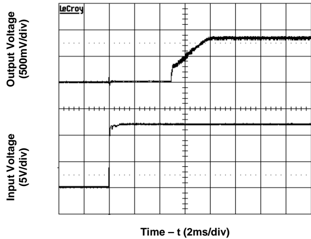
Figure 1d. Output Voltage (Vin=12V, full load)
