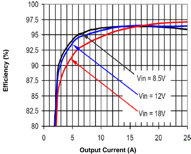
Figure 6a. Efficiency vs. Load Current (25°C)
