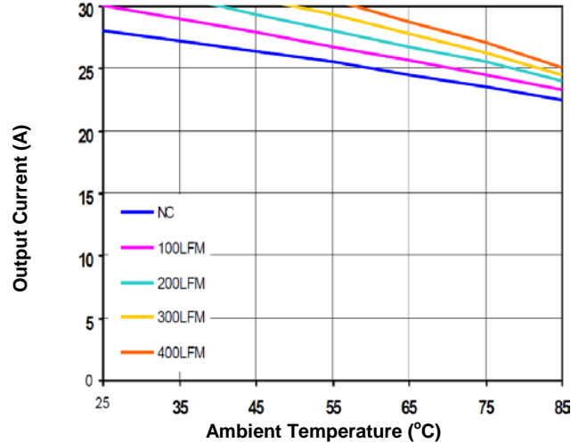
Figure 2b. Current Derating Curve ( V_{in}=12V , open frame)
