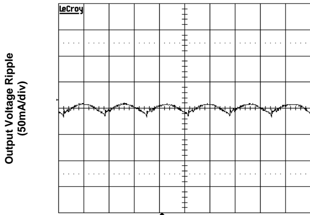
Figure 2c. Output Voltage (Vin=12V, full load)
