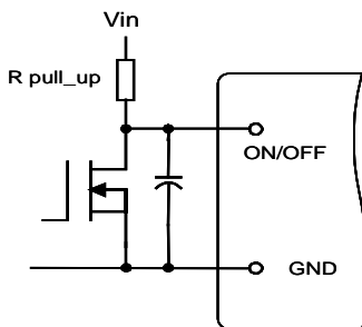
Figure 8. Circuit for Negative Logic Control
