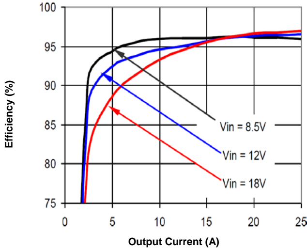
Figure 5a. Efficiency vs. Load Current (25°C)
