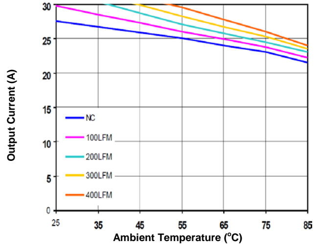
Figure 3b. Current Derating Curve ( V_{in}=12V , open frame)
