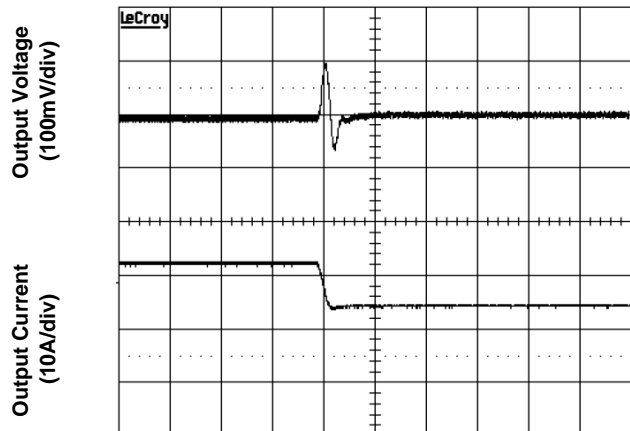
Figure 2d. Output Voltage (Vin=12V, full load)
