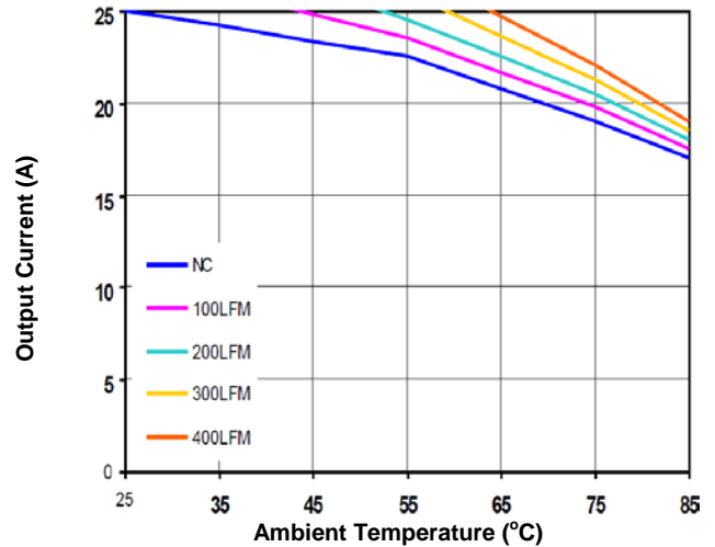
Figure 5b. Current Derating Curve ( V_{in}=12V , open frame)
