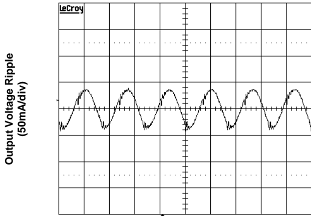
Time – t (2 \mu s/div) Figure 6c. Output Ripple Voltage ( V_{in}=12V , full load)
