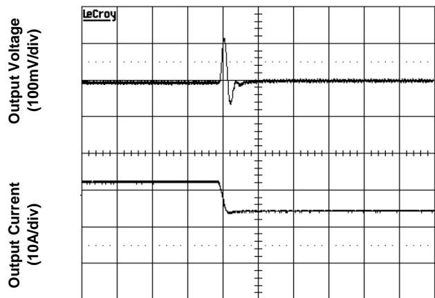
Figure 1d. Output Voltage (Vin=12V, full load)
