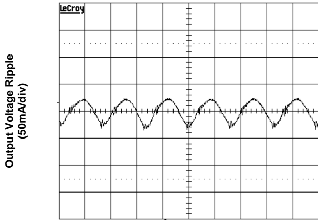
Time – t (2 \mu s/div) Figure 5c. Output Ripple Voltage ( V_{in}=12V , full load)
