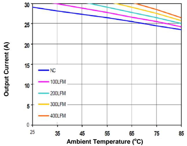
Figure 1b. Current Derating Curve (Vin=12V, open frame)
