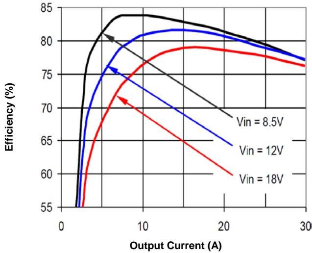
Figure 1a. Efficiency vs. Load Current (25°C)
