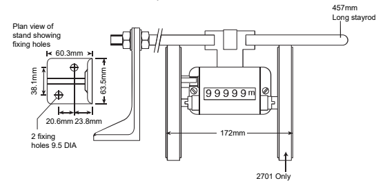
Product Dimensions 2401 | 2701
