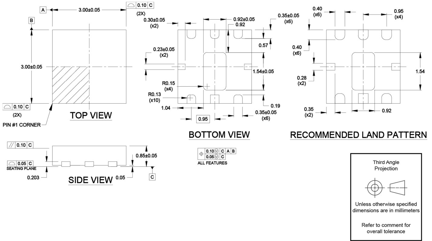
Figure 13. Package Drawing
