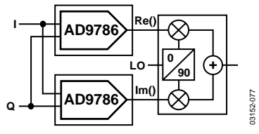
Figure 77. AD9786 Driving Quadrature Modulator
