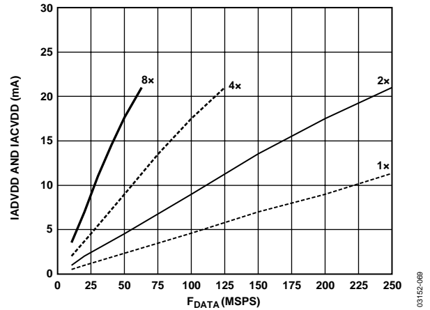
Figure 69. ADVDD and ACVDD Supply Current vs. Clock Speed and Interpolation Rates
