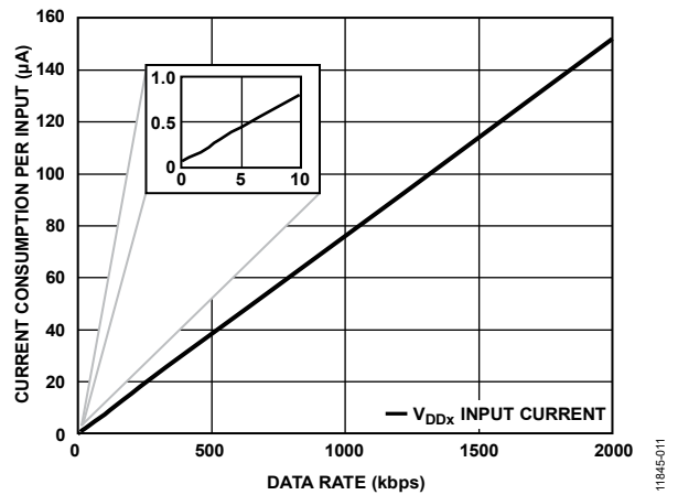
Figure 15. Current Consumption per Input vs. Data Rate for 2.5 V, EN_x = \text{High Operation}
