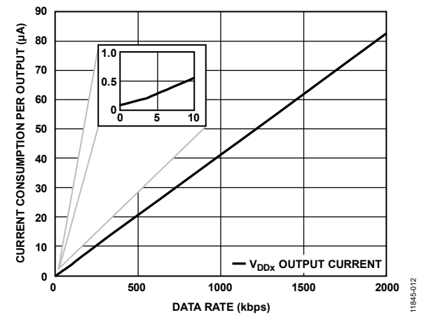
Figure 16. Current Consumption per Output vs. Data Rate for 2.5 V, EN_x = \text{High Operation}
