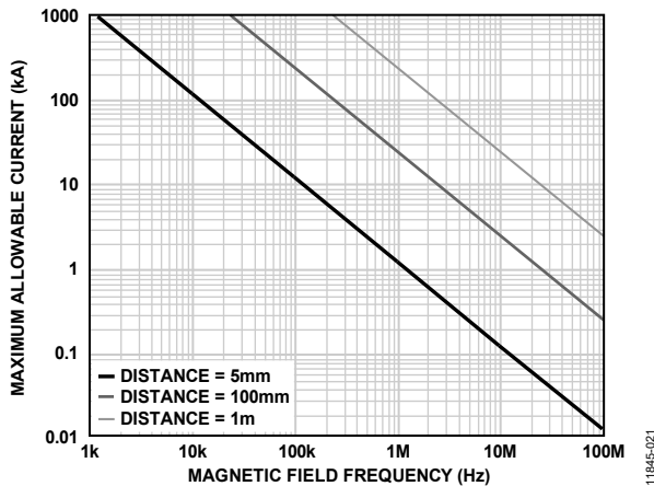
Figure 33. Maximum Allowable Current for Various Current-to-ADuM1440/ADuM1441/ADuM1442/ADuM1445/ADuM1446/ADuM1447 Spacings
