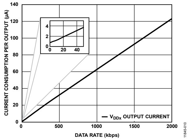
Figure 14. Current Consumption per Output vs. Data Rate for 3.3 V, EN_x = \text{Low Operation}
