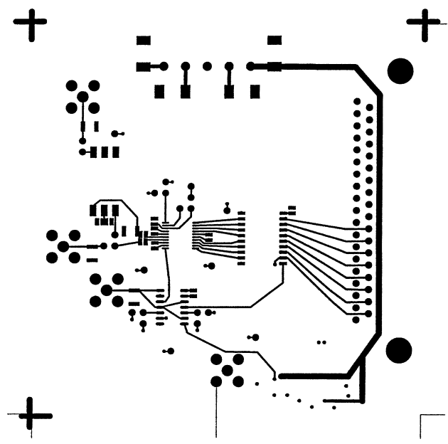
Figure 9. Printed Circuit Board Top Side Copper
