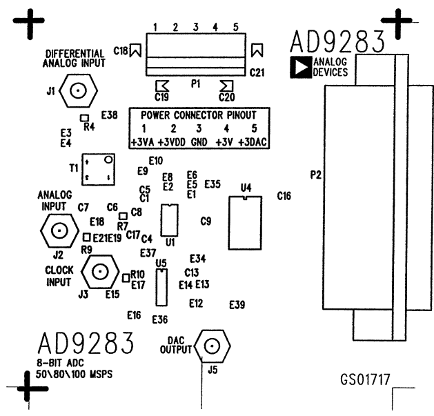
Figure 7. Printed Circuit Board Top Side Silkscreen
