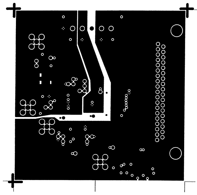
Figure 10. Printed Circuit Board "Split" Power Layer
