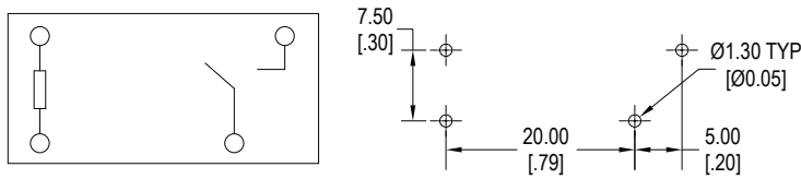
Version 2, 1A, 5.0mm Terminal Spacing
