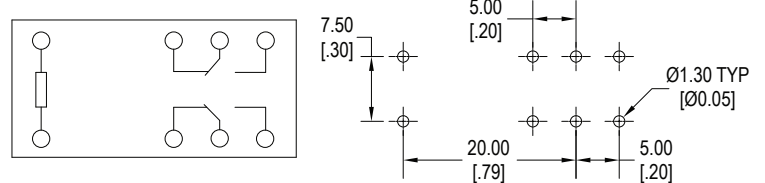
Version 4, 2C, 5.0mm Terminal Spacing
