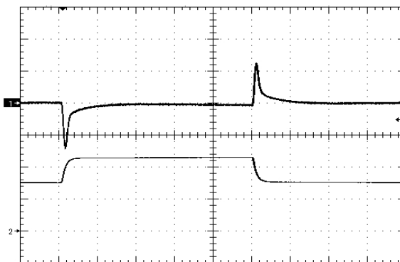
Figure 12. Load Transient Response (100mV/div), di/dt=0.1A/µS, 50%-75%-50% of full load, Cout=Fig16 time scale: 200µS/div. Ch1=Vout, Ch2=Iout (1A/div)
