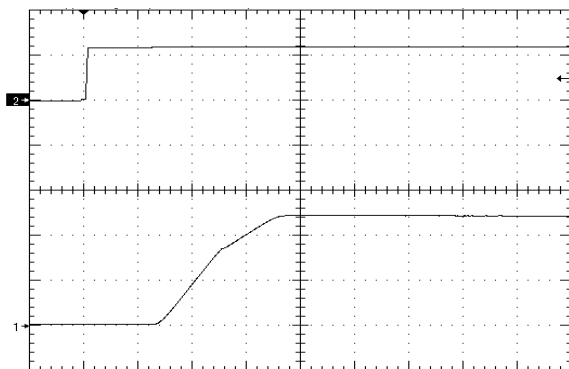
Figure 11. Startup Waveform via Enable Pin, time scale 4mS/div. Vin=Vin_nom, Iout=full load Cout=1000µF, Ch1=Vout (2V/div), Ch2=enable (5V/div)
