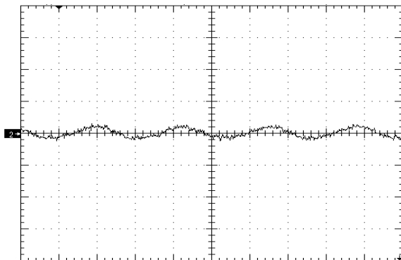
Figure 7. Input Reflected Ripple Current (10mA/div), time scale – 1µS/div. Vin=Vin_nom, full load (see Fig 15)
