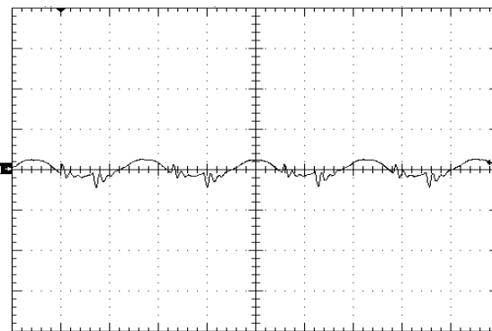
Figure 8. Output Voltage Ripple (50mV/div), time scale – 1µS/div. Vin=Vin_nom, full load Cout=1µF ceramic + 10µF Tantalum (see Fig 16)
