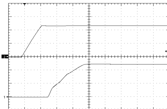
Figure 10. Startup Waveform via Input Voltage, time scale 4mS/div. Vin=Vin_nom, Iout=full load Cout=0µF, Ch1=Vout (2V/div), Ch2=Vin (20V/div)
