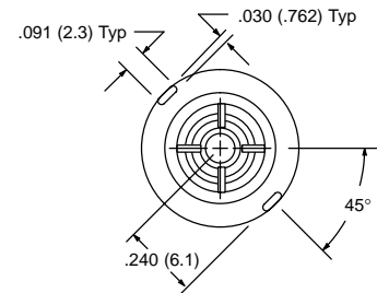
Shaft End
