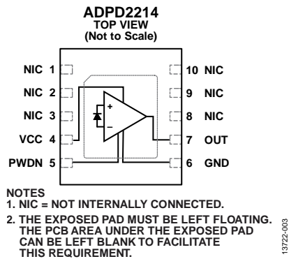
Figure 3. Pin Configuration
