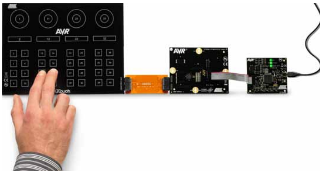
Figure 8 – Complete set-up for the Atmel® QMatrix 8x8 sensor board: The sensor board is connected to the Atmel ATmega324, which in turn is connected to the interface board
