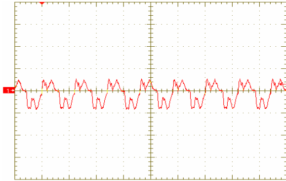
Figure 7. Output Voltage Ripple (50mV/div), time scale – 2uS/div.
