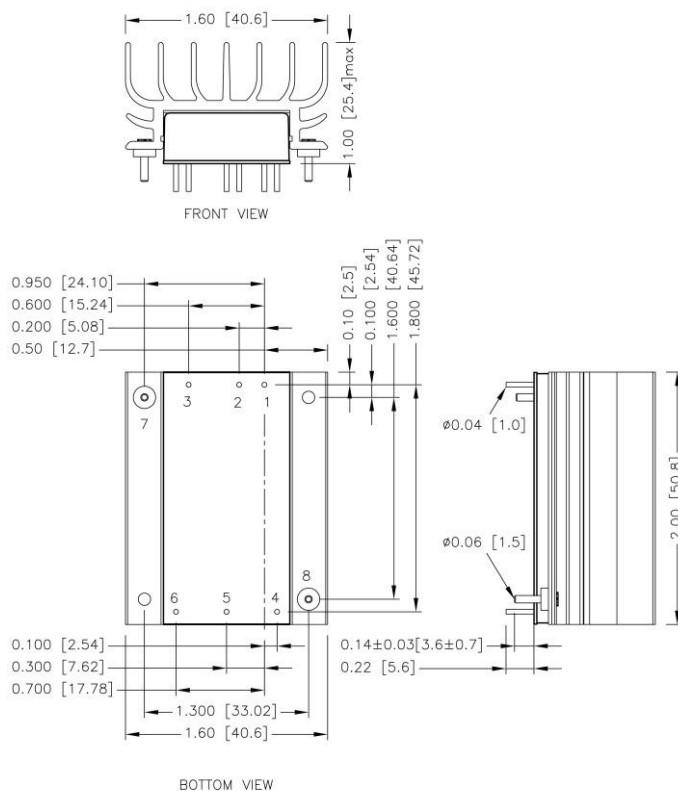
BOTTOM VIEW
