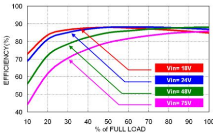
FED30-48T0515W Efficiency vs. Output Load
