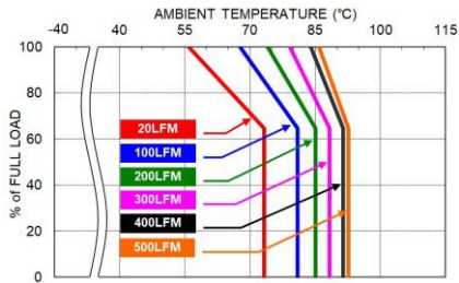
FED30-48T0515W Derating Curve
