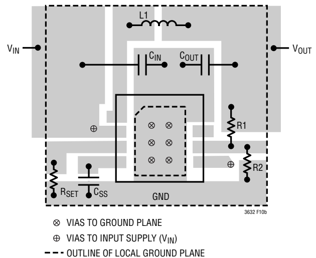
Figure 10. Layout Example
