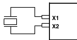
FIGURE 11. RECOMMENDED CRYSTAL CONNECTION
