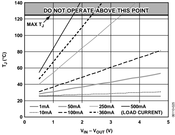
Figure 37. 0 mm 2 of PCB Copper, T_A = 25^\circ\text{C}
