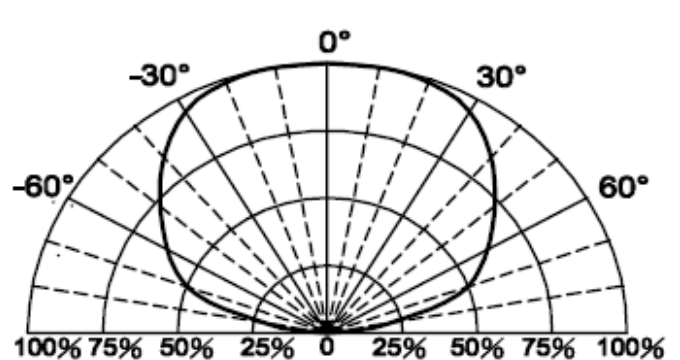
Fig.6 Directivity Radiation
