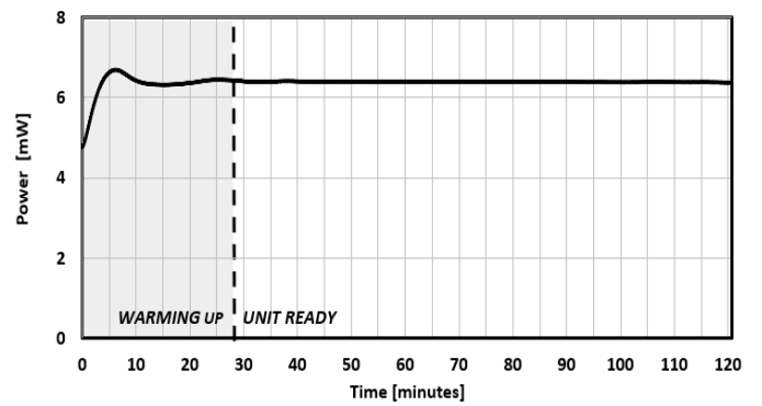
FIG. 4: WARM-UP TIME
