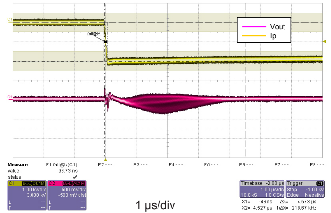
Figure 14: dv/dt
