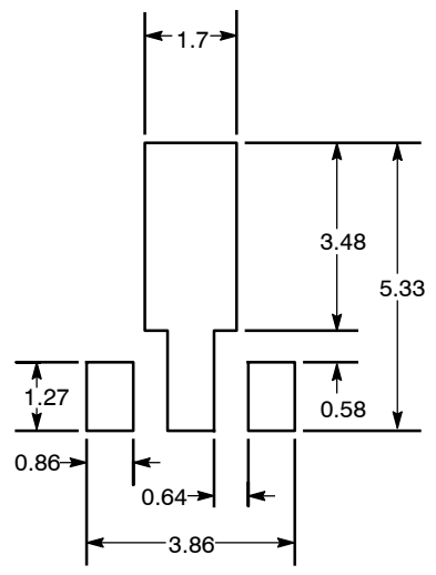
Recommended Solder Stencil
