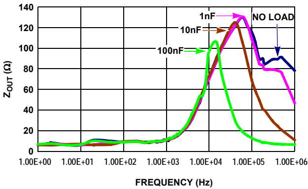
FIGURE 52. Z OUT vs FREQUENCY
