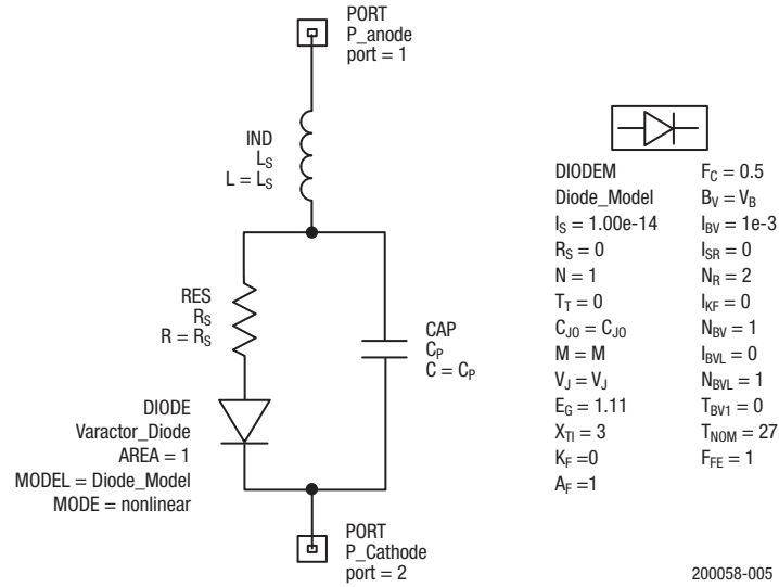
Figure 5. SPICE Model
