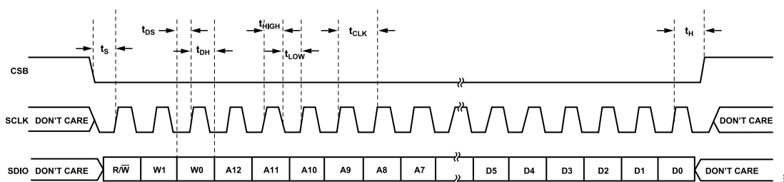
Figure 68. Serial Port Interface Timing Diagram
