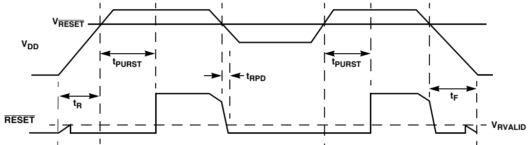
FIGURE 4. RESET TIMING
